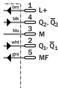
5-polig, M12
