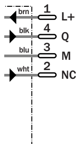
5-polig, M12
