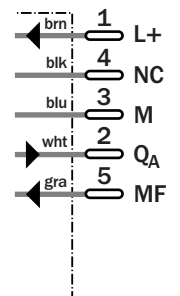
5-polig, M12
