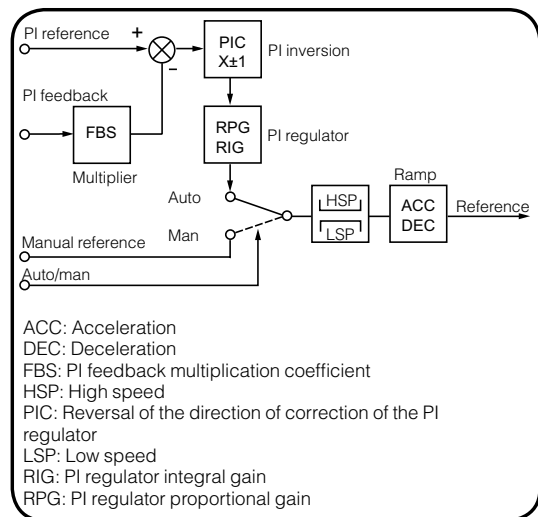
PI feedback
