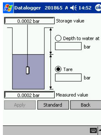
Configuration of Datalogger e.g. storage rate, sample rate, offset (tare) etc.
