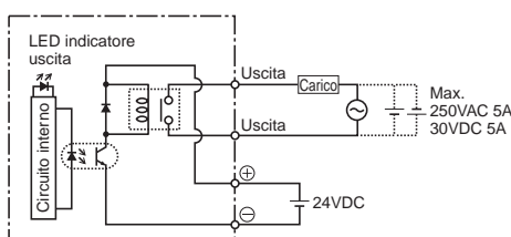
FP2-Y6R
