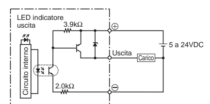
FP2-Y16P
