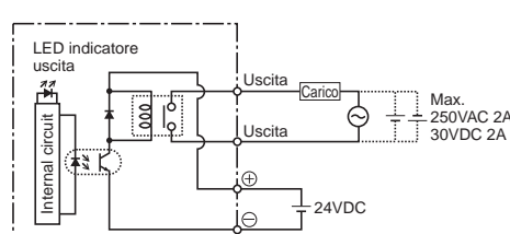
FP2-Y16R
