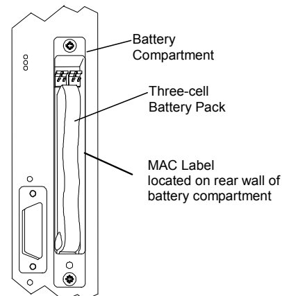
Figure 2. Battery Compartment
