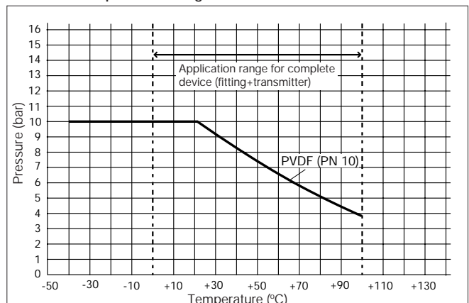
Pressure-Temperature-Diagram
