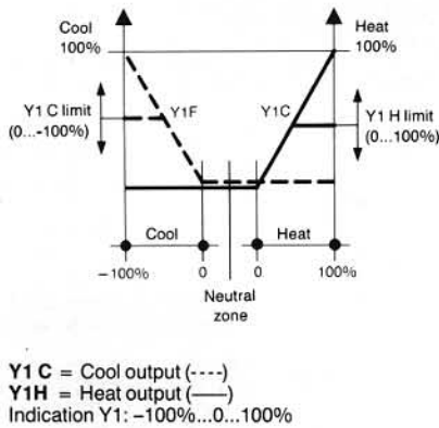
Fig. 3: Output characteristic for dual action controllers. Example: Heat-Cool
