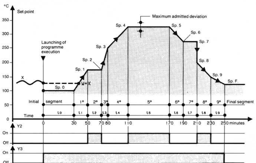
Fig. 4: Example of Programmed Set point
